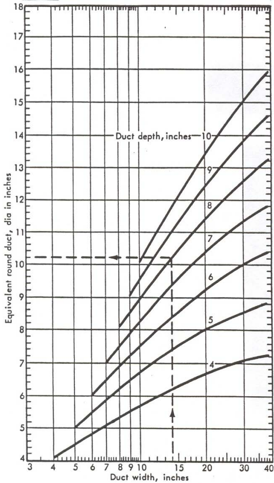
1 Circular equivalent of rectangular duct for equal velocity
