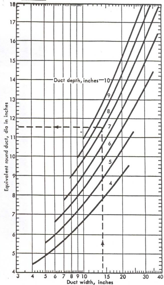
2 Circular equivalent of rectangular duct for equal capacity
