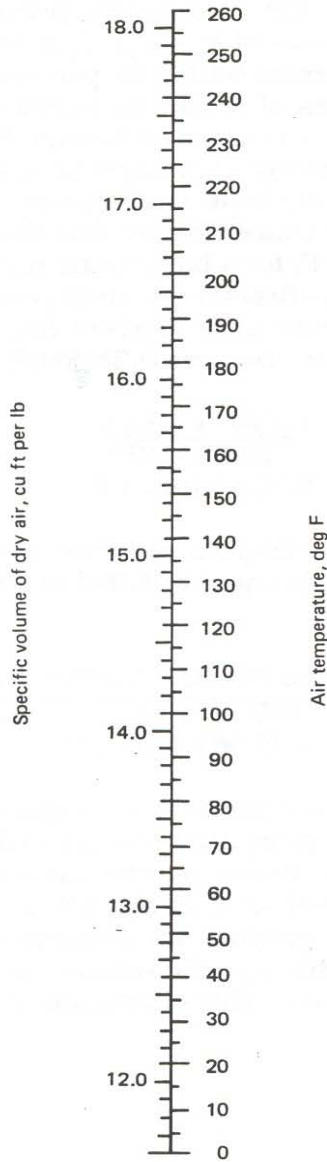
Figure 1. NOMOGRAPH yields specific volume (reciprocal of air density) of dry air for dry bulb temperatures from zero to 260° F assuming standard barometric pressure.
